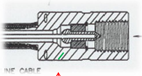
Original design with heat buildup area existing
